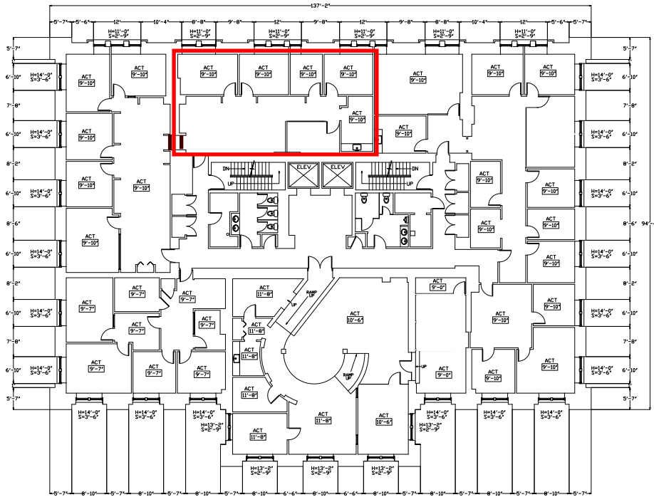
2 EXISTING SECOND FLOOR PLAN
